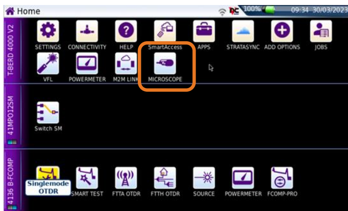
Figure 4: Home Screen
